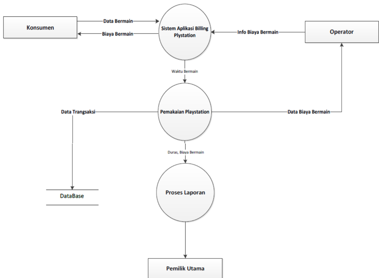
Gambar 3. DFD Level 0
