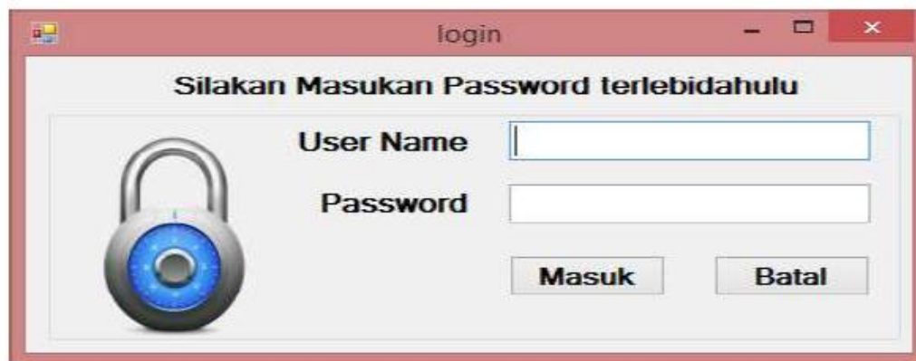
Gambar 9. Form Login
